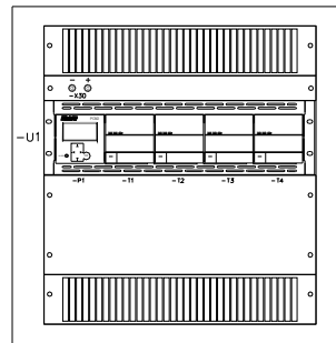
PRM1 in wall cabinet, PRM1-W
