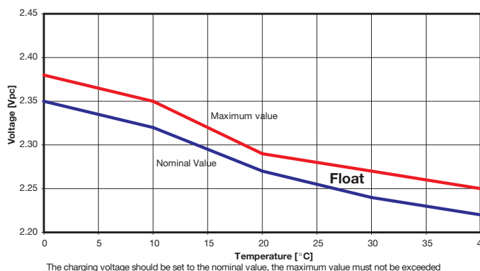
Fig. 1: Marathon L and Powerfit S; charging voltage vs. temperature
